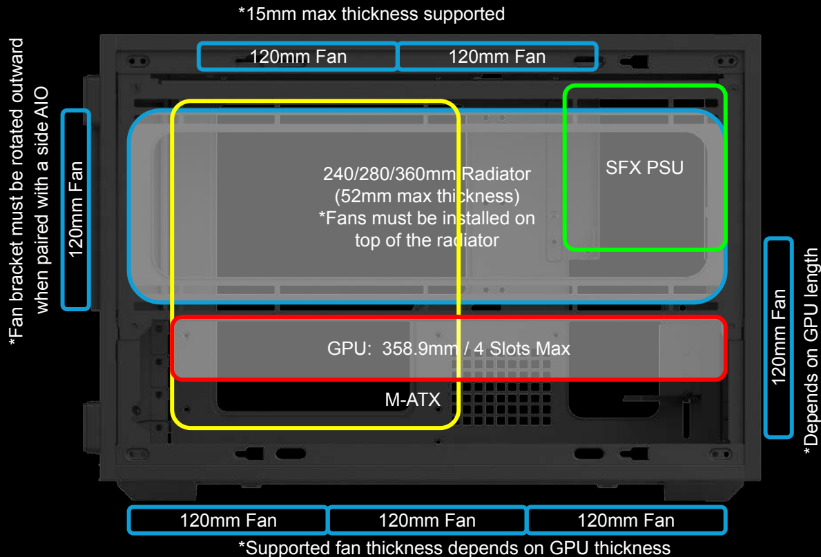
With SFX PSU
