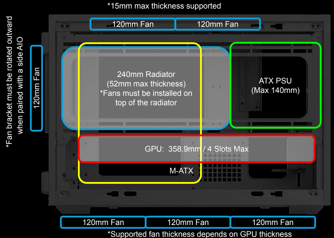
With ATX PSU
