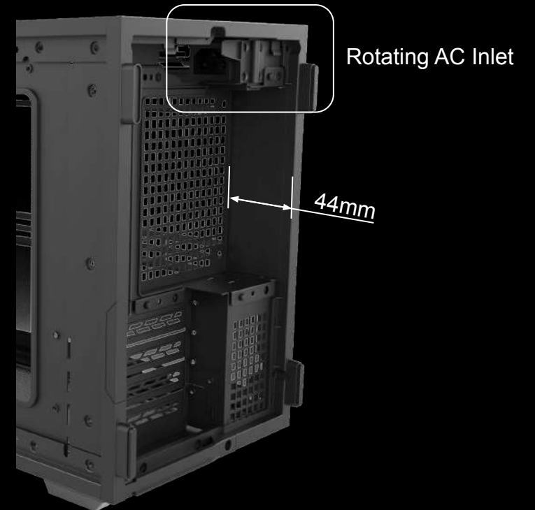
Spacious Rear I/O SPACE
