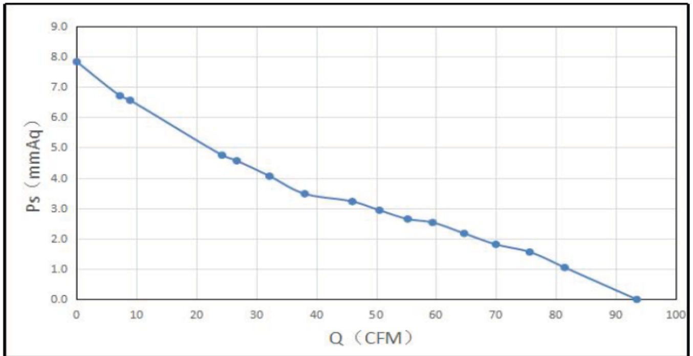
P-Q Curve
